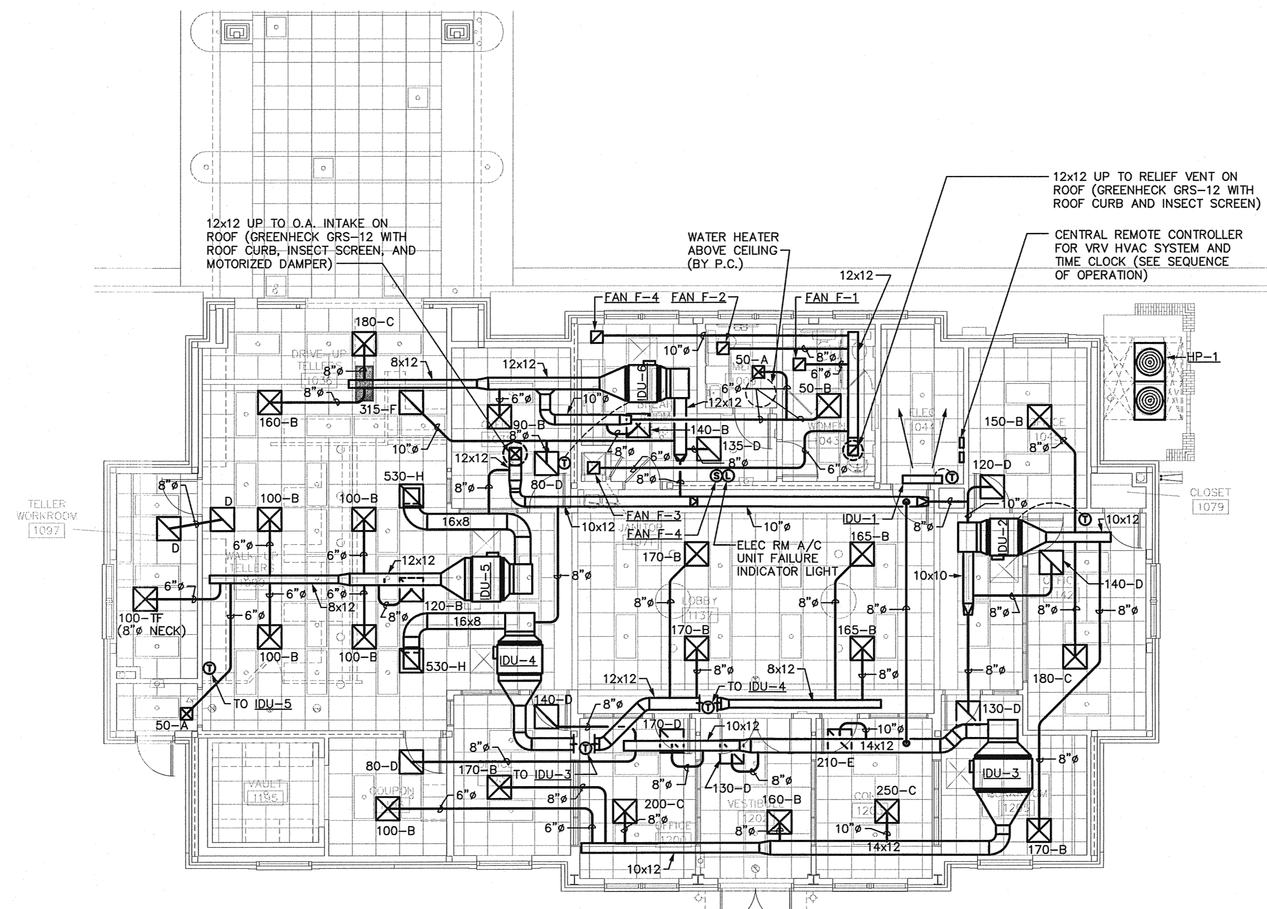
1 FLOOR PLAN - MECHANICAL 1/8" = 1'-0"
