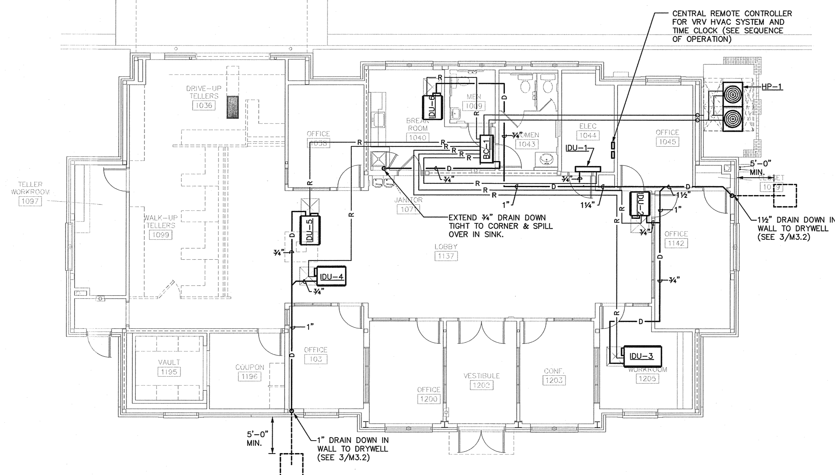
1 PIPING PLAN - MECHANICAL 1/8" = 1'-0"
